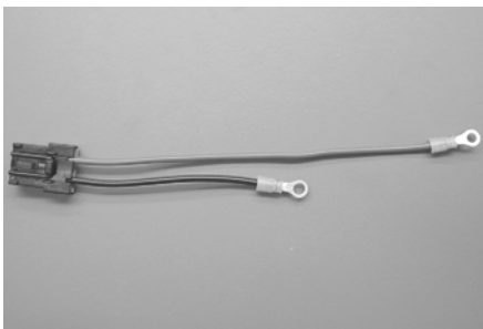
94-639 Walbro GSS pump connector to ring terminals. Wire is 14 AWG. Overall length is 7". Used in pump and kit #'s GCA317, GCA355, GCA3305, GCA3318, GCA3322, GCA3323, GCA3325, GCA3338, GCA3341, GCA3357, GCA3369, GCA3381, GCA3384 and GCA764.
