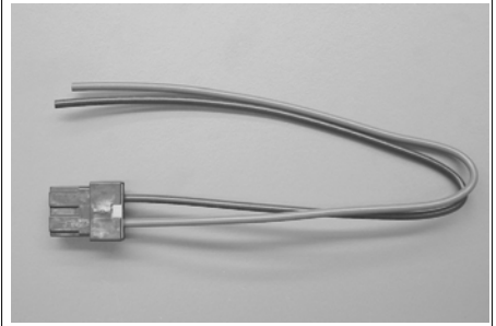
94-615 Universal wire harness with Walbro GSS pump connector on one end. Wire is 14 AWG. Overall length is 12". Use with 187-113 butt connectors. Use in pump & kit #'s GCA311,
