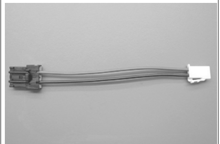
94-646 Walbro GSS pump connector to Mitsubishi style connector. Polarity is reverse of 94-614. Wire is 16 AWG. Used in pump and kit #'s GCA343, GCA3342 and GCA3390.
