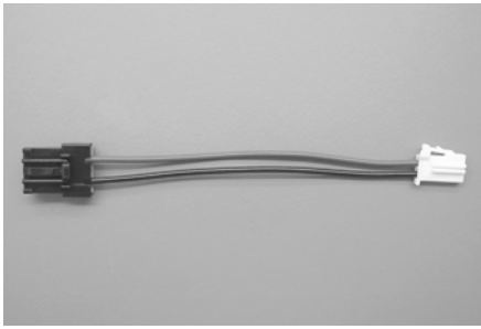
94-614 Walbro GSS pump connector to Mitsubishi style connector. Wire is 16 AWG. Overall length is 7". Used in pump and kit #GCA702.
