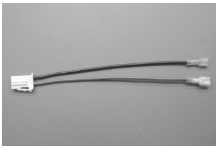
94-638 Female spade connectors to Mitsubishi style connector. Wire is 16 AWG. Overall length is 7". Used in pump and kit #'s TCA318 and TCA380.
